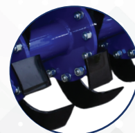
Helical blade fitment for better load distribution.
